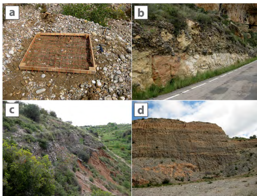
Fig. 3. Quaternary fluvial terrace deposits: a) sampling frame for 1 m 2 test pits; b) level Qt 3 covering Eocene limestones of Cinglera de la Cascalda-Roca dels Bous; c) level Qt 6 covering Oligocene strata (near the town of Camarasa); d) level Qt 6 , gravel deposit (near the town of Camarasa).
