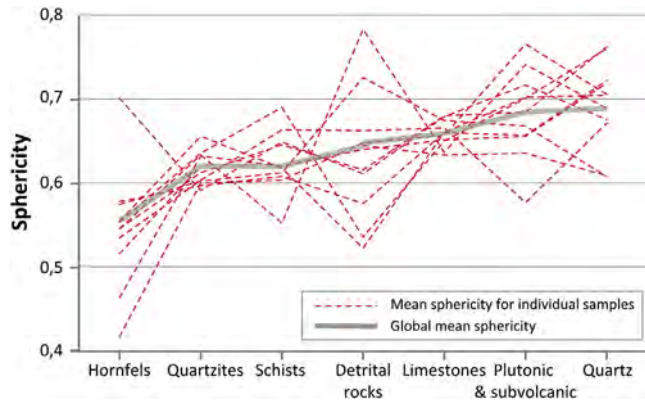
Fig. 6. Evolution of average sphericity of different rock types.
